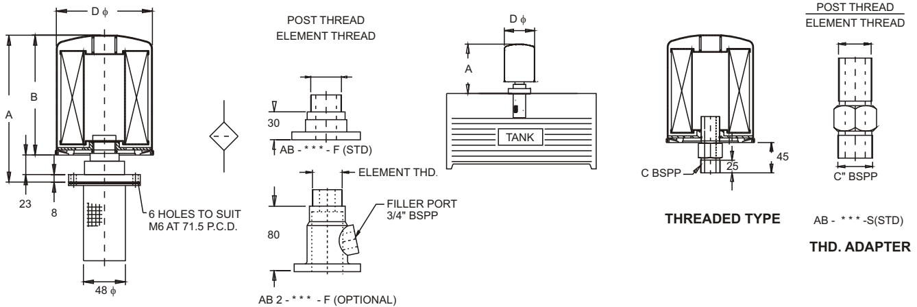
FLANGE TYPE
