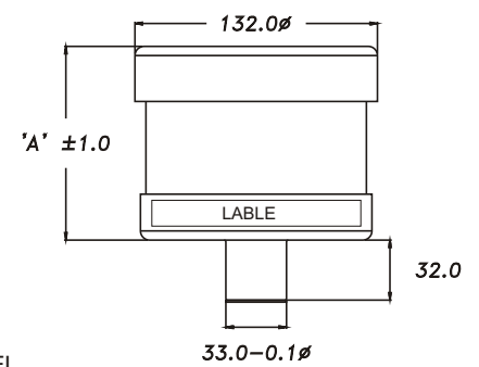
PIPE MOUNTING - DBP ( To Suit 1-5/16" Id Pipe )
