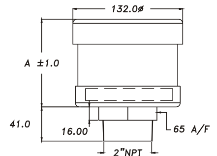
THREAD MOUNTING - DBT
