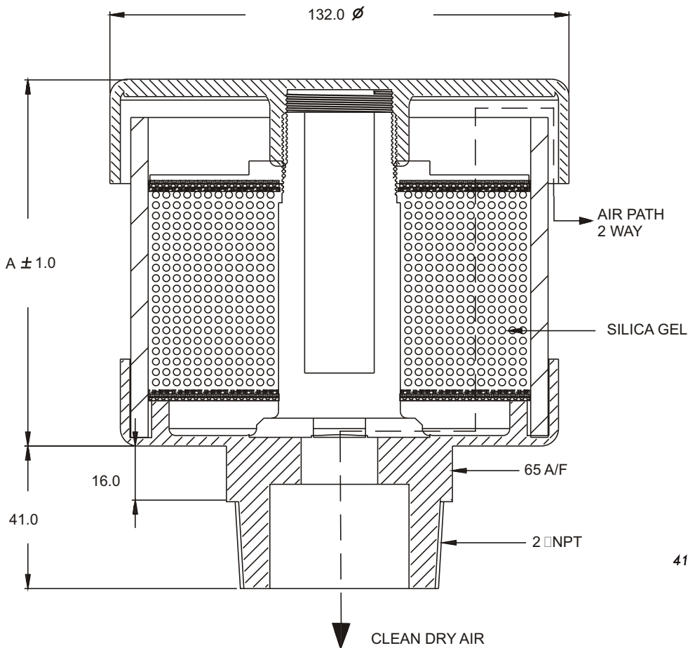
THREAD MOUNTING - DBT
